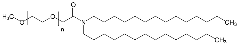
Figure 3.2.A.3.1.2-1. Chemical Structure of ALC-0159
